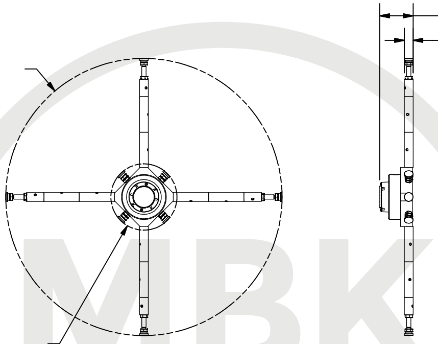
ID Bearing Mount Assembly For ID diameters of 11.25 - 47 inches (285.8 - 1193.8 mm)
