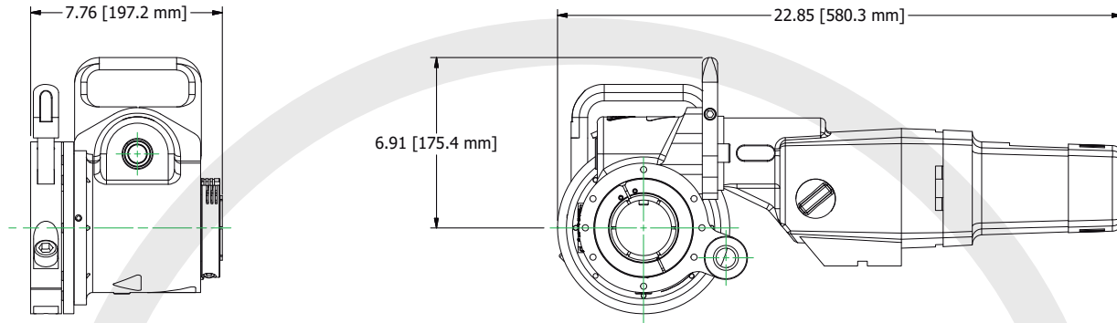
Rotational drive unit with electric motor
