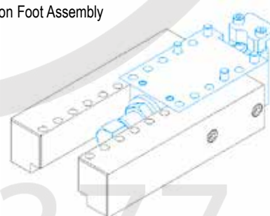
Extension Foot Assembly
